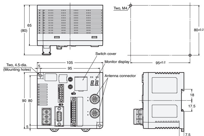
Mounting Hole Dimensions
